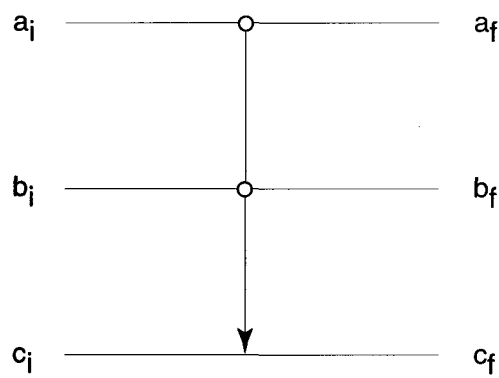
Figure 9.2: The graph for the CCN-gate.
