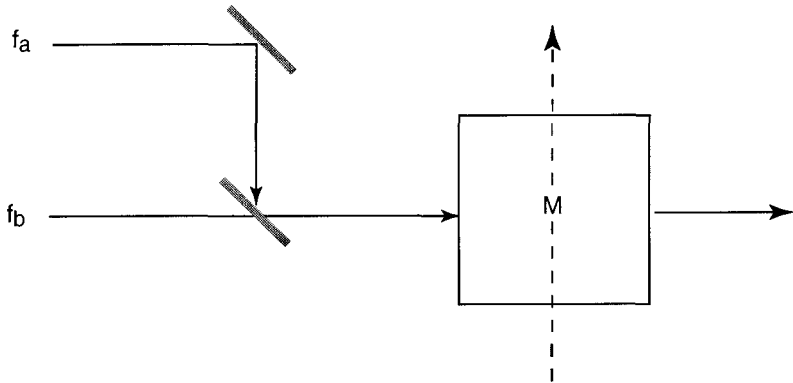
Figure 23.2: Scheme of the experiment [24]. Two photon beams with frequencies f_a and f_b interact in the cavity M via an atom. The dashed line shows the atomic beam.
