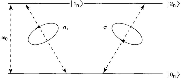
Figure 18.1: Energy levels of the n -th ion. States |1_n\rangle and |2_n\rangle can be driven independently by laser beams with different polarization; \omega_0 is the frequency of the optical transition.
