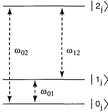
Figure 13.1: The third auxiliary level, |2_j\rangle , is used to implement the A_j transformation.
