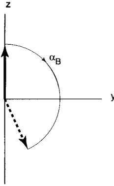
Figure 24.3: Rotation of spin B around the x -axis of the rotating frame under the action of the distorted \pi -pulse.
