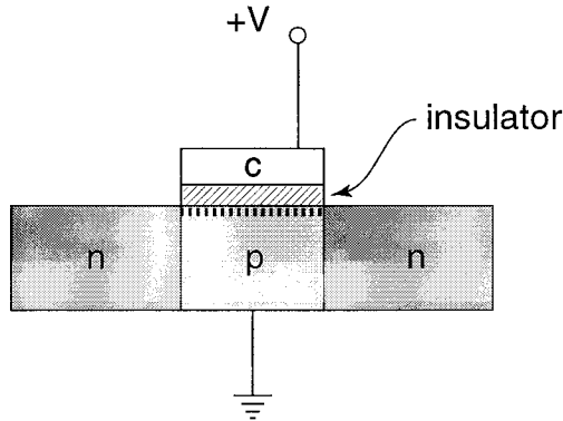
Figure 8.2: Metal-oxide-semiconductor-field-effect-transistor (MOSFET); p is a p -type semiconductor, n are the n -type semiconductors, c is the conductor. Symbol \equiv means a connection to the ground.
